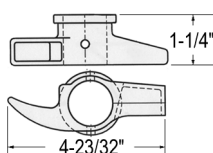
Upper Lock Rod Cam
