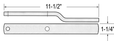
Door Latch Handle
