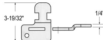
Door Latch Tongue
